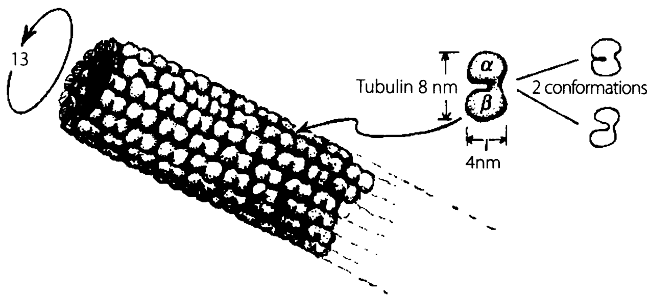
Fig. 4a. A microtubule. It is a hollow tube, normally consisting of 13 columns of tubulin dimers. Each tubulin molecule is capable of (at least) two conformations
